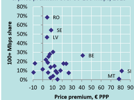
Figure 14: 100+ Mbps share of BB in covered areas & price premium over 30-100 Mbps, 2015 101
